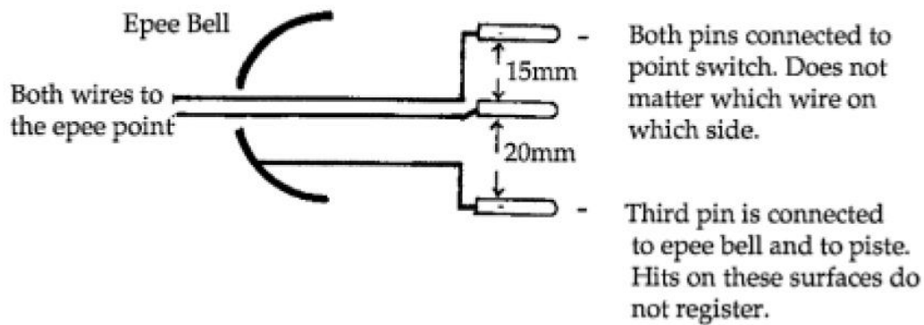
FIG. 9 EPEE SCORING AND GROUND CIRCUITS
