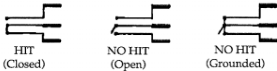
Fig. 10 EPEE HIT REGISTRATION (SCHEMATIC)
